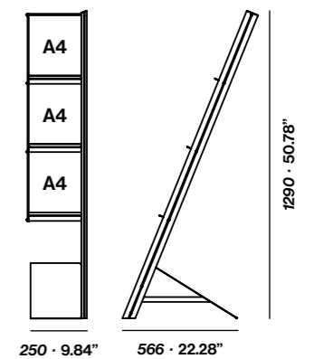
IFT Triple with shelf · Triple con repisa
